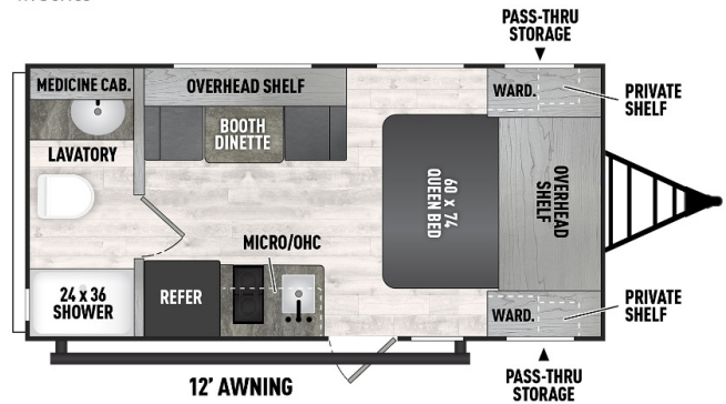
18FQ FLOORPLAN 4K Series
